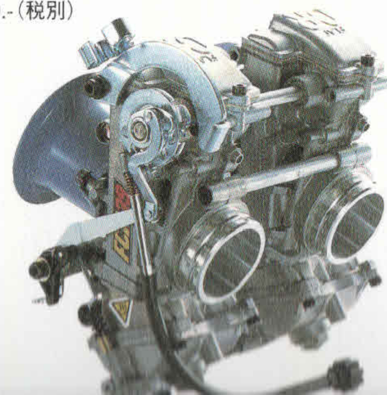
JB-POWER FCRφ28 MONKEY (H/Z) ¥50,000.- (税別)
