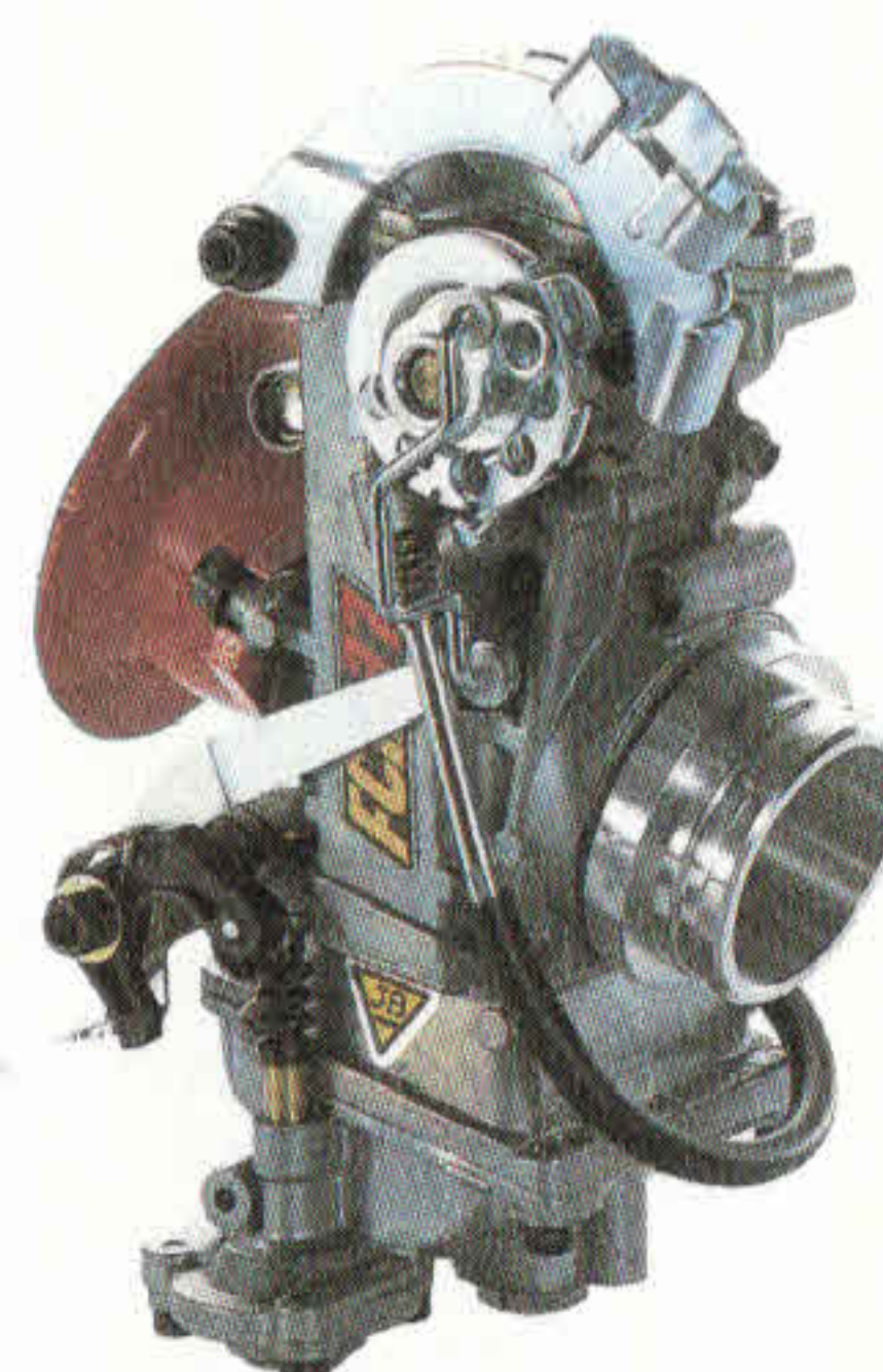
JB-POWER FCRφ28 MONKEY (H/Z) ¥50,000.- (税別)
