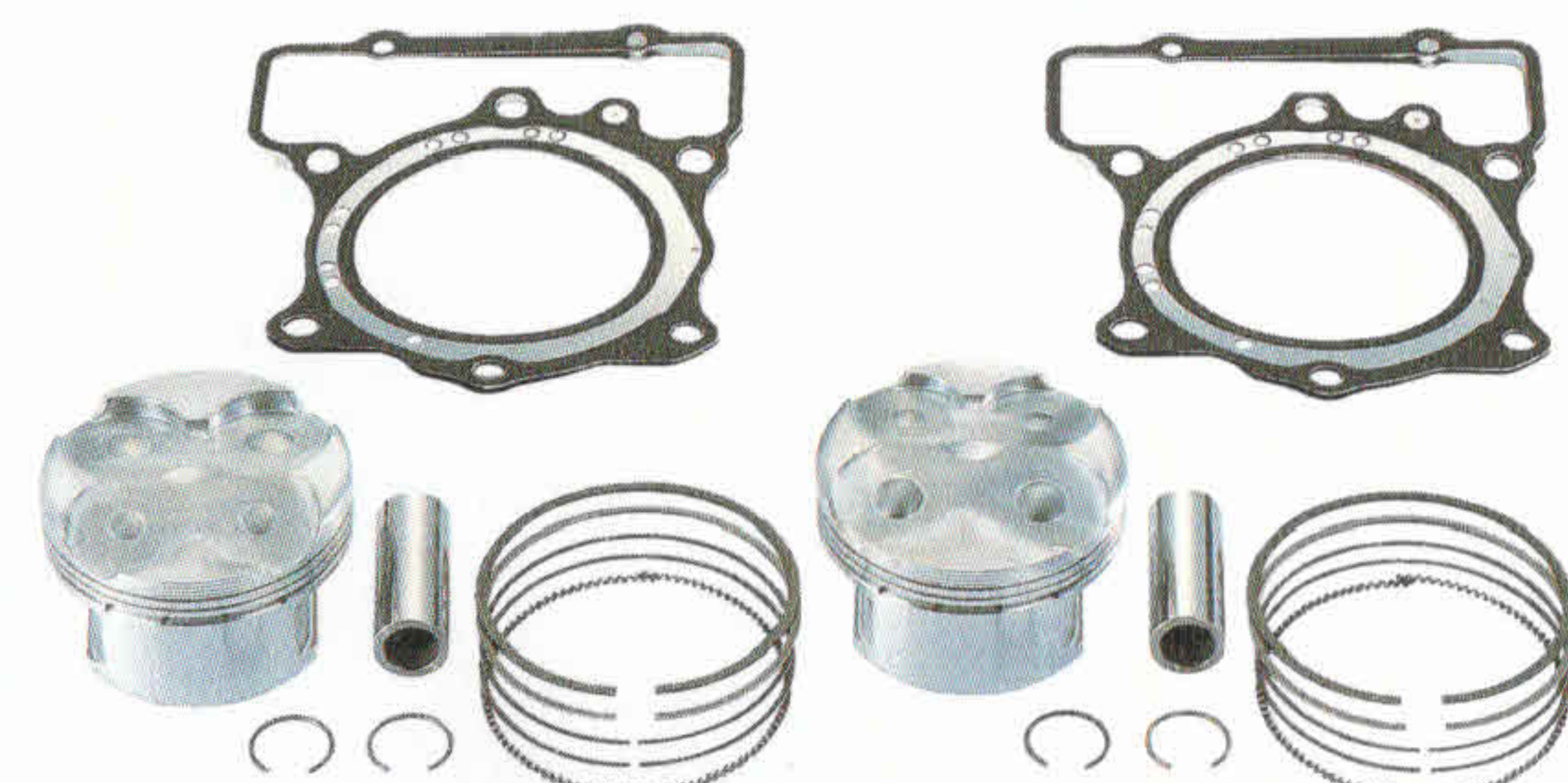
JB-POWER COSWORTH \phi 98 VTR1000F ¥93,000.- (税別)
